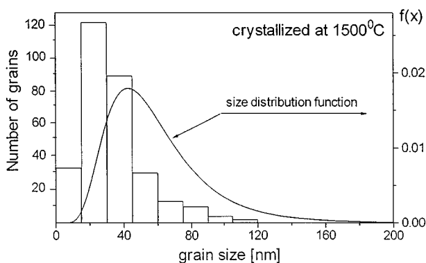
Figure 6 Bar-diagram of the size distribution obtained from TEM micrographs and the size distribution function, f(x) (solid line), determined by X-rays for powder heat-treated at 1500°C.
