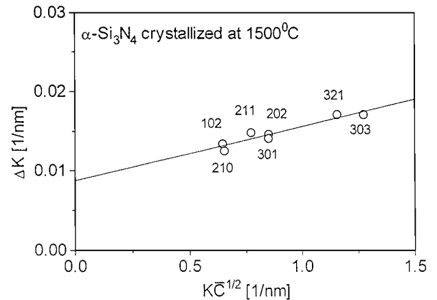
Figure 1 The FWHM as a function of K \bar{C}^{1/2} for \alpha - \text{Si}_3\text{N}_4 in powder crystallized at 1500°C according to the modified Williamson-Hall plot in Equation 1. The Miller indices of the reflections are also indicated.
