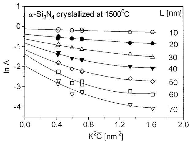
Figure 3 The logarithm of the real part of the Fourier coefficients versus K^2 C , for \alpha -Si 3 N 4 in powder crystallized at 1500°C according to the modified Warren-Averbach plot in Equation 3.
