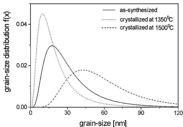
Figure 5 The grain-size distribution function, f(x) , of the crystalline fraction of the as-synthesized powder and the samples heat-treated at 1350 and 1500°C.
