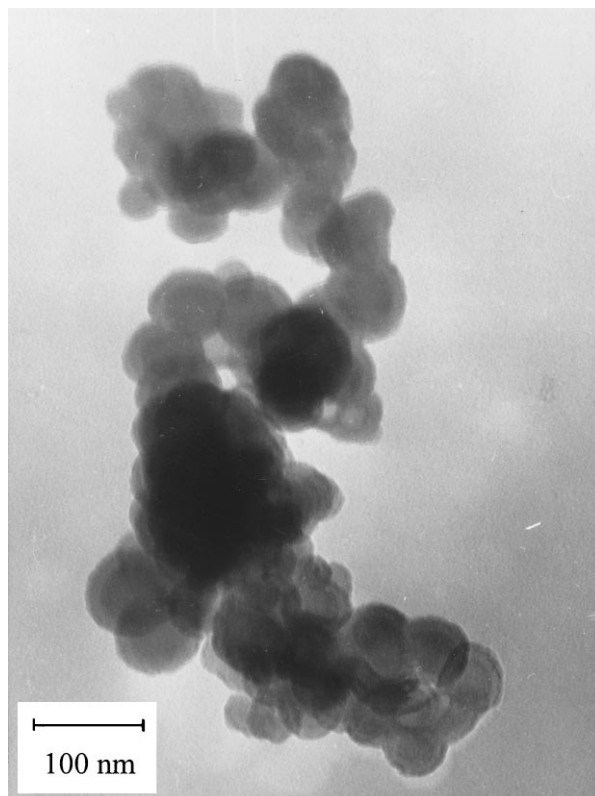
Figure 7 TEM micrograph of powder crystallized at 1500°C.
