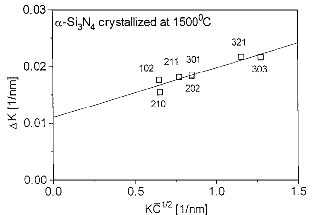
Figure 2 The integral breadth as a function of K \bar{C}^{1/2} for \alpha - \text{Si}_3\text{N}_4 in powder heat-treated at 1500°C according to the modified Williamson-Hall plot in Equation 1. The Miller indices of the reflections are also indicated.
