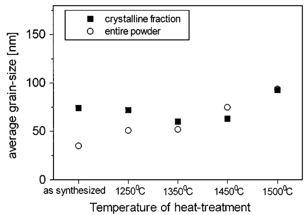
Figure 4 The area-weighted average grain-size of the crystalline fraction and that of the entire powder heat-treated at different temperatures.
